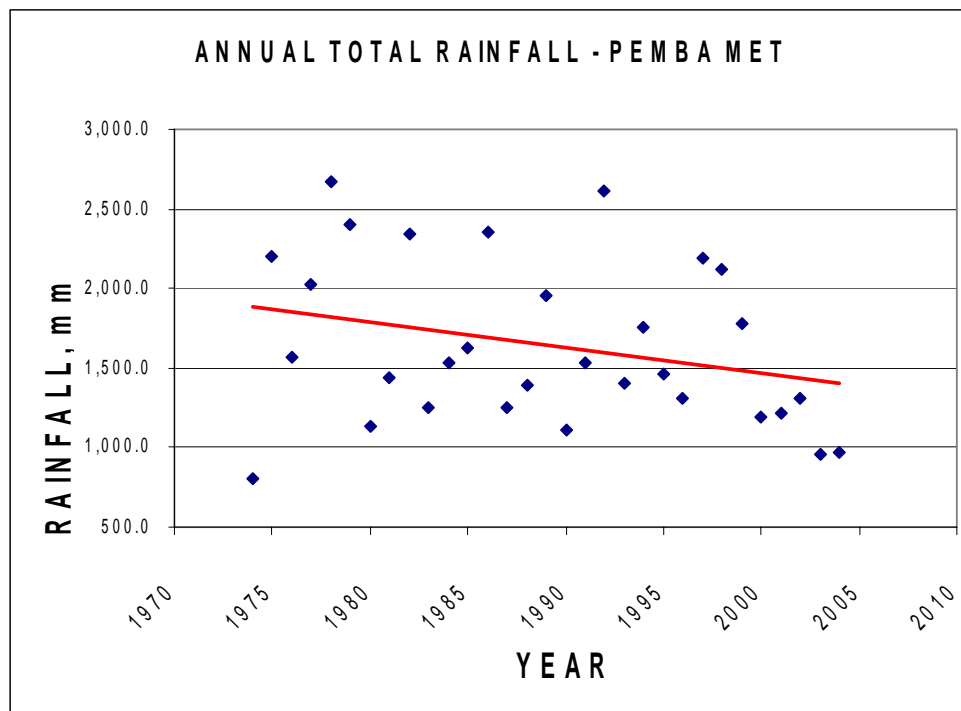
Figure 4: Rainfall Pattern at Pemba Meteorological station
